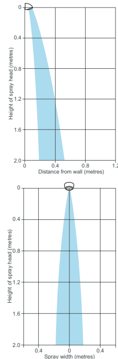
Spray Patterns at 9 l/min
