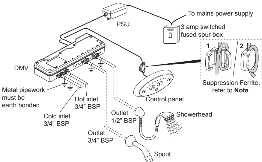
Installation Schematic
